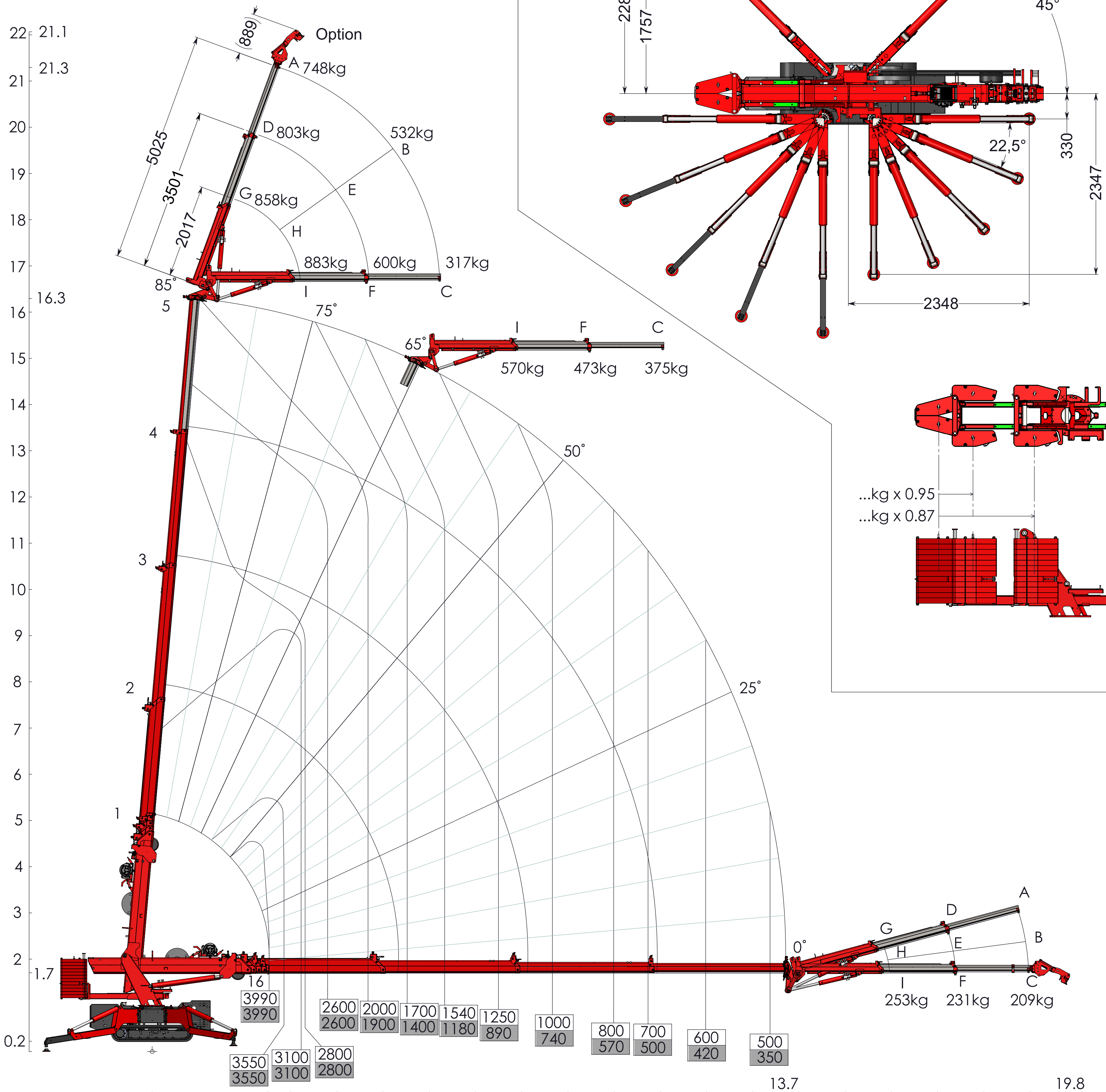
C10 Load diagram v1.4_26-10-20
