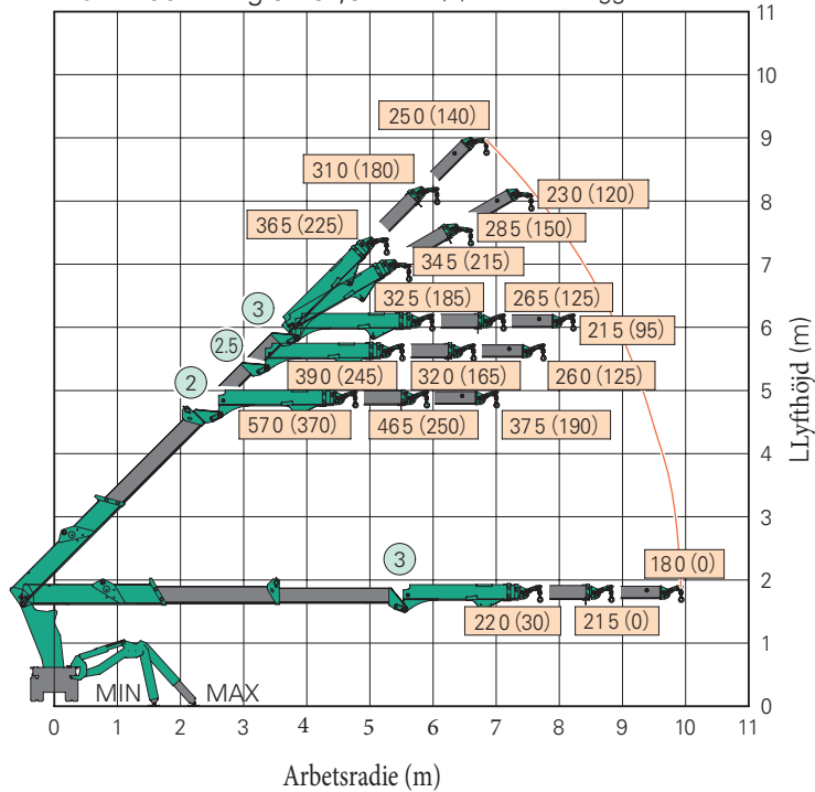
Main Boom Angle 45°, 0° ( ) = MIN Outriggers Position
