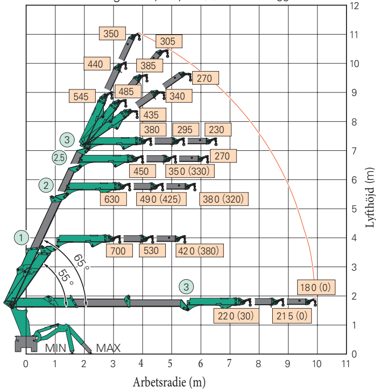
Main Boom Angle 65°, 55°, 0° ( ) = MIN Outriggers Position
